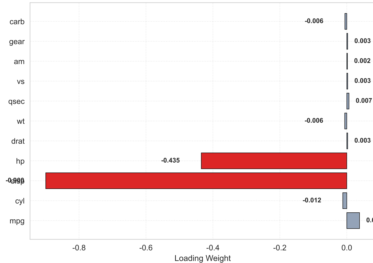
(A) Unstandardized PC1 Loadings (Dominated by 'disp' & 'hp')
