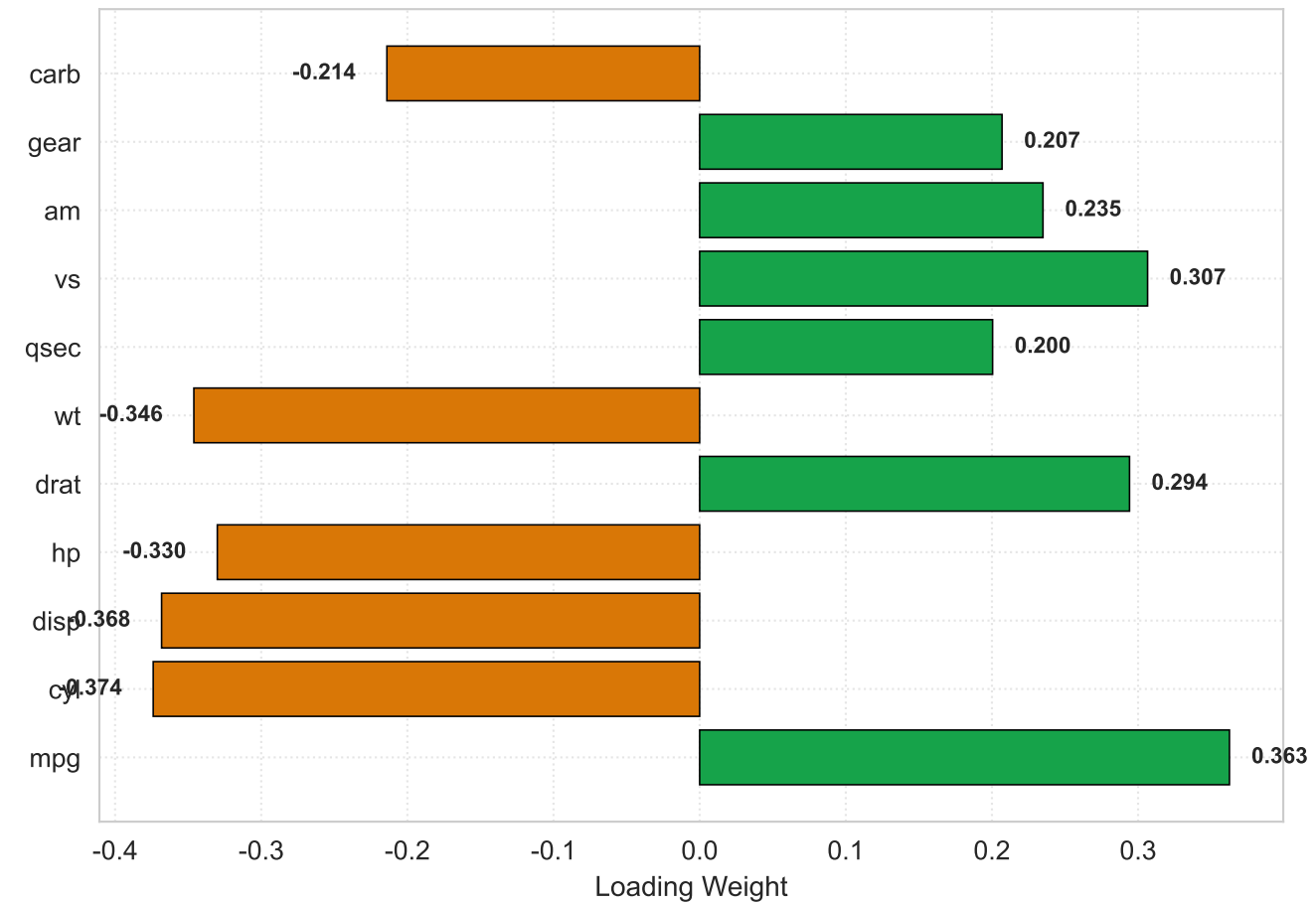
(B) Standardized PC1 Loadings (Balanced Multi-Feature Representation)
